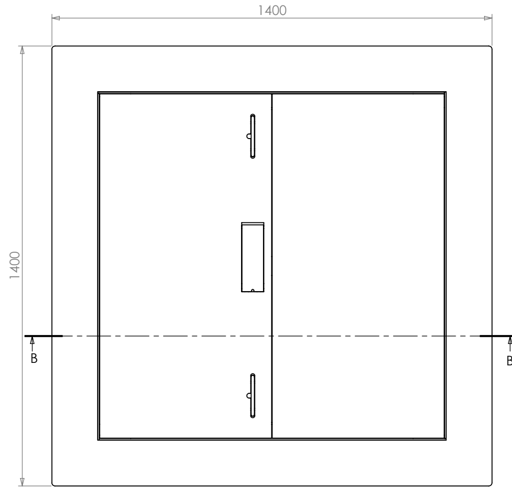
TOP VIEW
